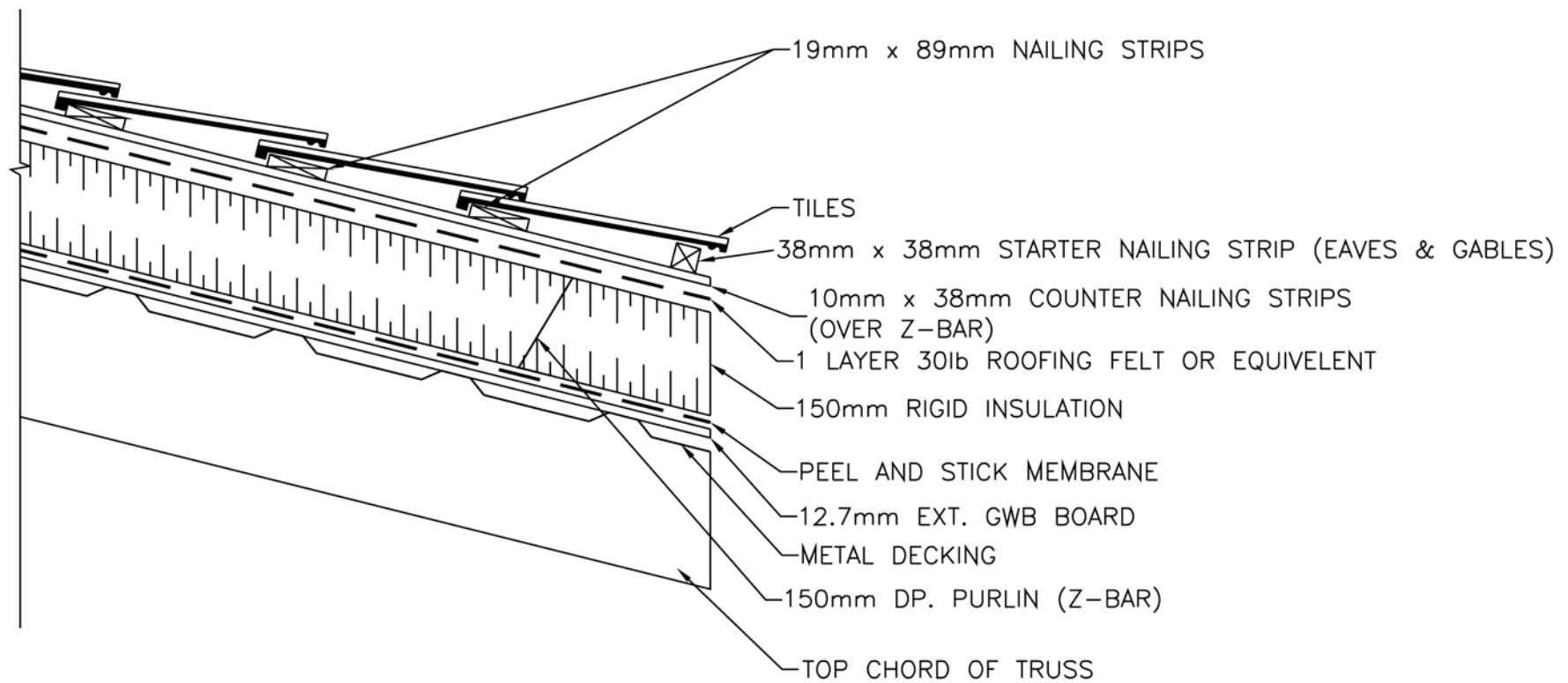
NON-COMBUSTIBLE ROOF DETAIL SCALE 1:10
